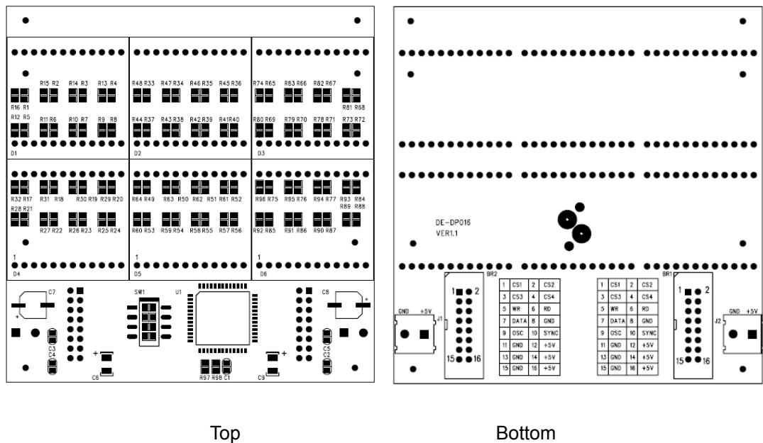
Figure 4 PCB Layout
